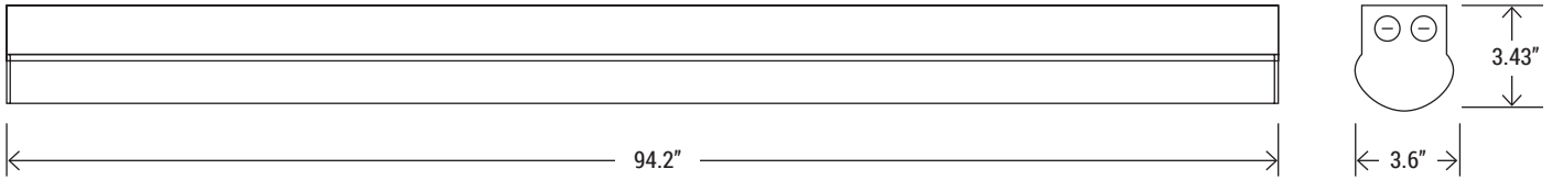
8' PT-LSFA Series
