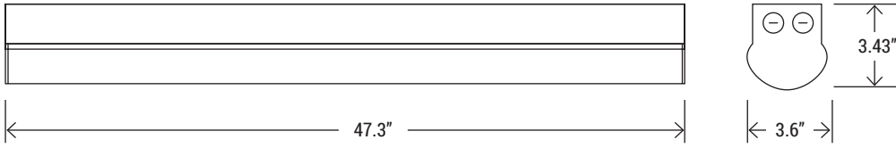
4' PT-LSFA Series
