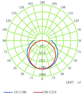
LUMINOUS INTENSITY DISTRIBUTION DIAGRAM
