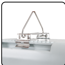
Suspension V-hook brackets (two provided)
