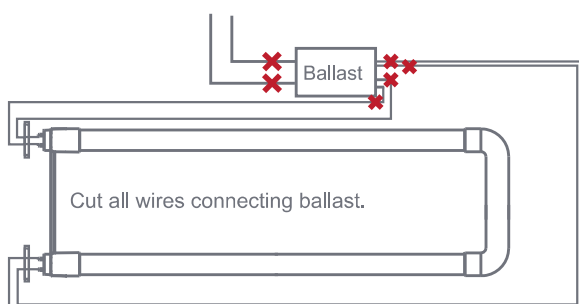
Diagram 1 – Cut all ballast wires
