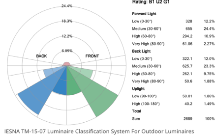
BUG rating
