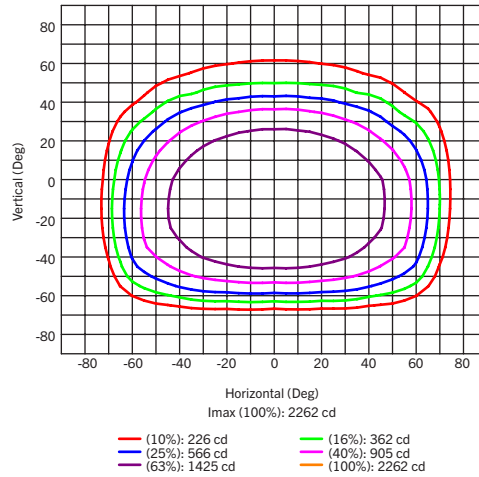
Isocandela (Rectangle)
