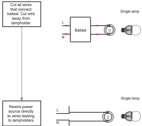
Diagram 2 – Fixture with ballast wiring modification
