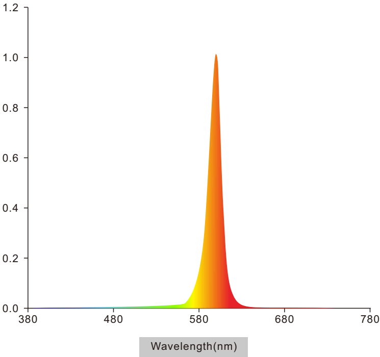
Spectrum
